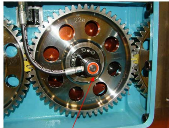
New Rotary Systems Rotary Union: C10179
