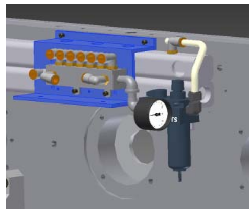
Fixed Base Air Distribution
