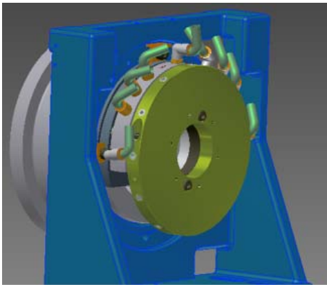
Fixed Base Manifold
